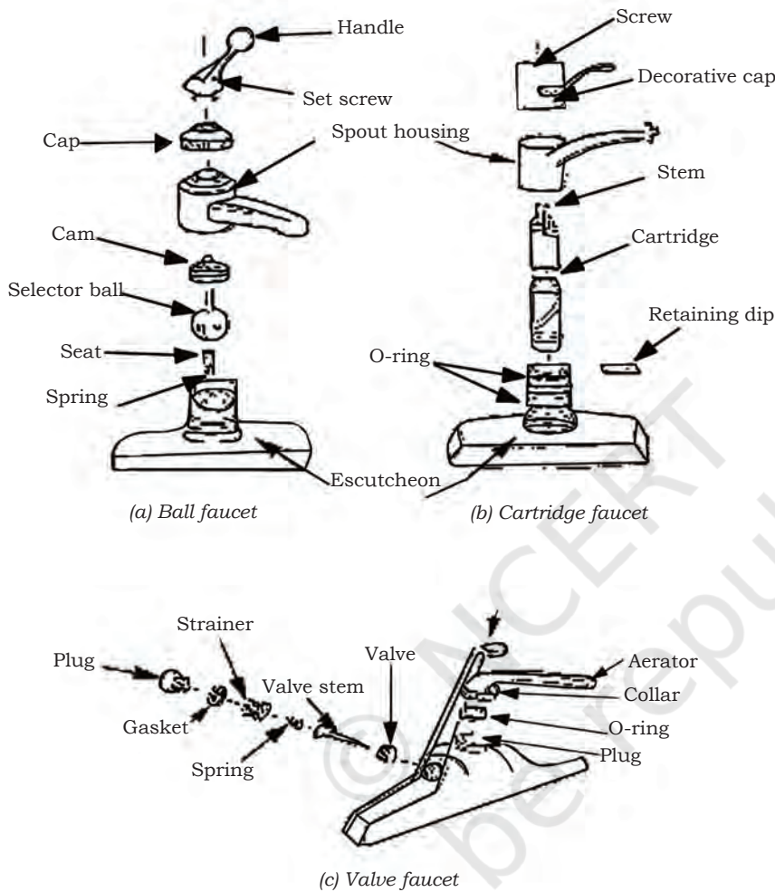
Fig. 5.2 (a, b, c) Components of faucets
