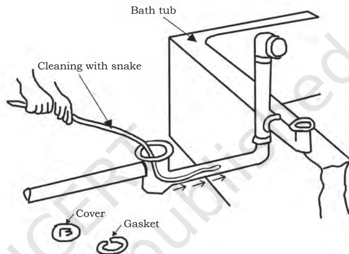
Fig. 5.14: Cleaning bath drum-trap stoppages
