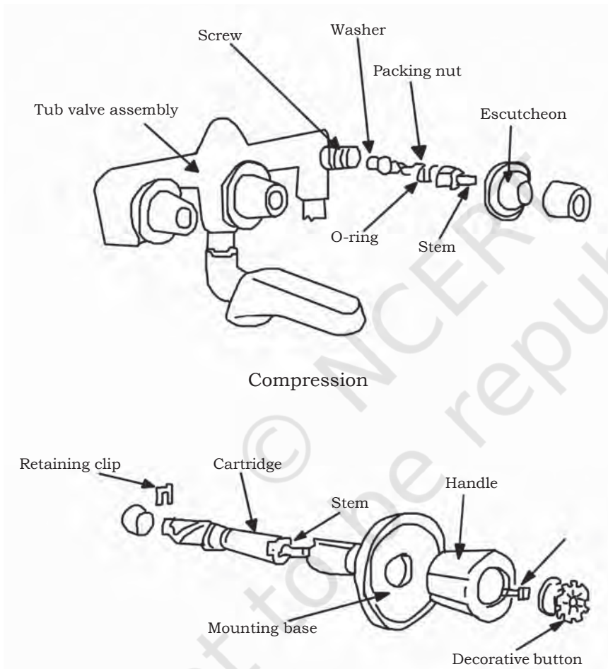
Fig. 5.7: Bathtub faucet breakout
